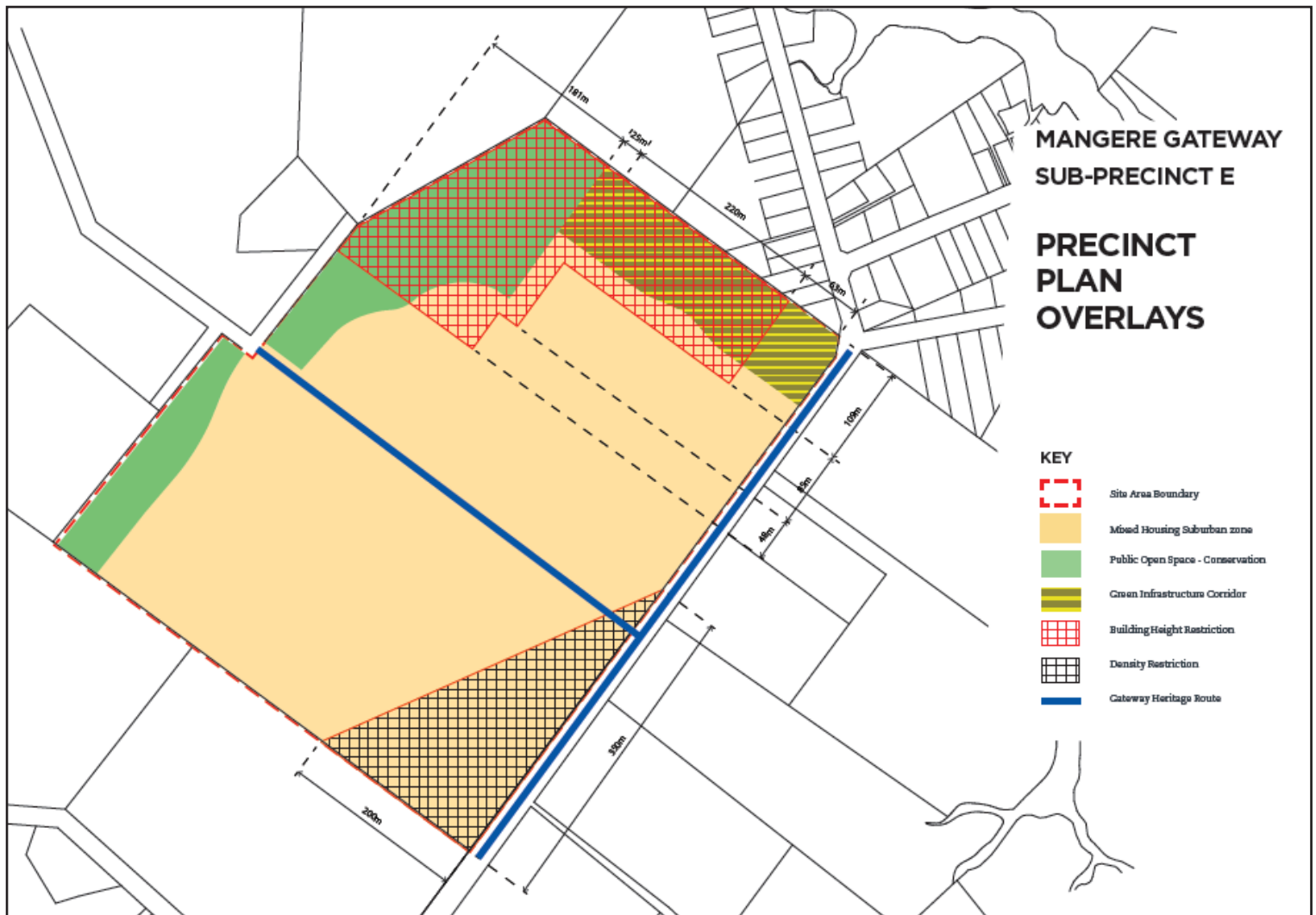
Figure 3 - Precinct Plan 2
